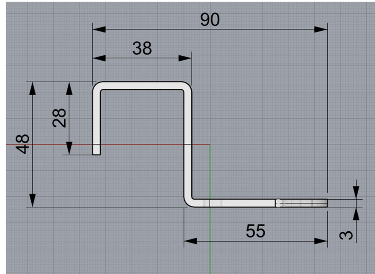
Bracket 3 Side View
