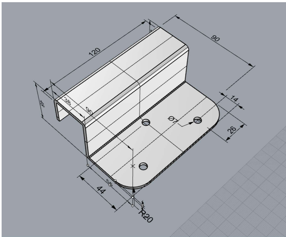
Bracket 3 Perspective View
