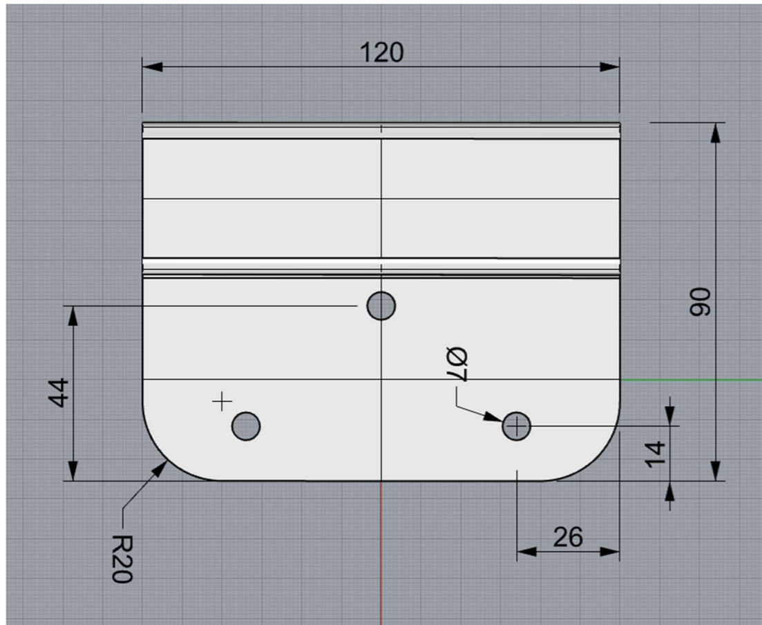
Bracket 3 Top View
