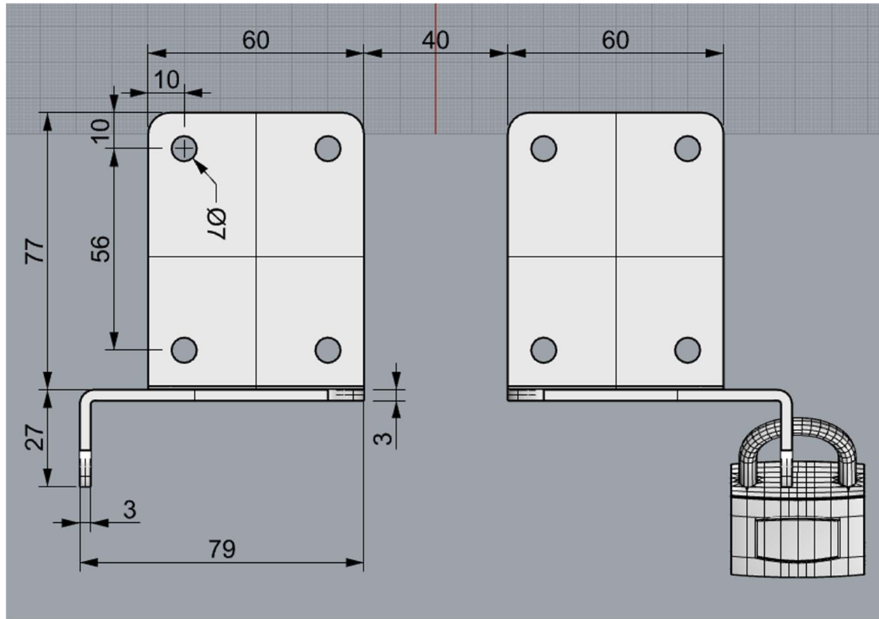
Bracket 1 & 2 Top View
