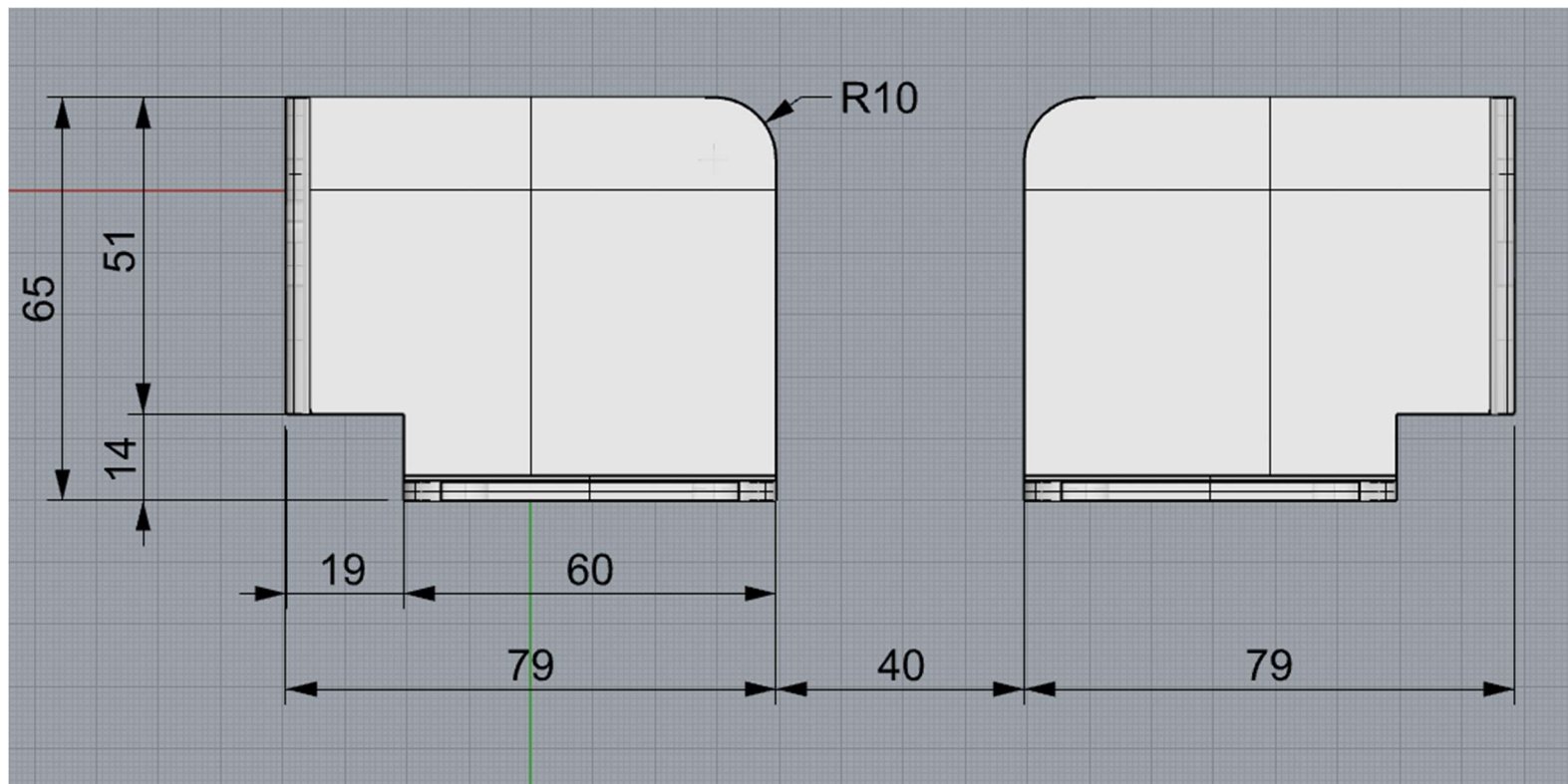
Bracket 1 & 2 Front View
