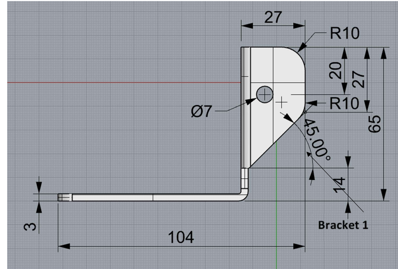
Bracket 1 & 2 Side View
